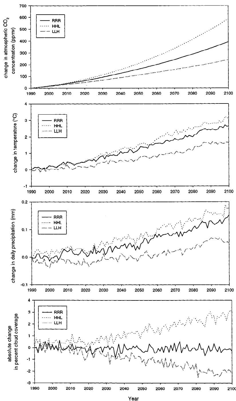
Figure 3. Transient changes in global mean annual atmospheric CO 2 concentration, global mean annual temperature, global mean daily precipitation and global mean annual percent cloudiness over the period of 1990–2100, projected by the coupled two-dimensional atmospheric chemistry/land-ocean climate model in the MIT Integrated Global System Model (see Figure 1 and Prinn et al. , 1998). The graph is presented using their values in 1990 as the reference.
