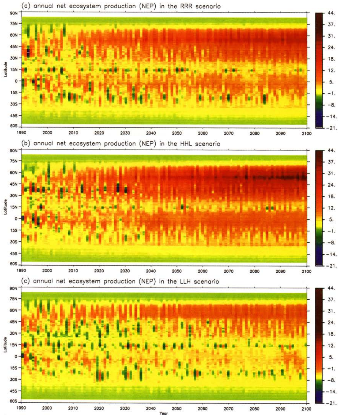
Plate 2. Latitudinal distributions of annual net ecosystem production (NEP) ( 10^{12} g C yr ^{-1} ) along 0.5^{\circ} -resolution latitudinal bands over the period of 1990–2100 in the RRR, HHL, and LLH transient climate change predictions.
