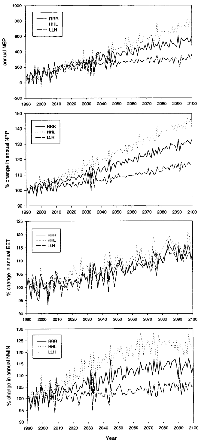
Figure 5. Temporal changes in annual net ecosystem production (NEP) ( 10^{12} g C \text{yr}^{-1} ), net primary production (NPP), net nitrogen mineralization (NMIN), and estimated evapotranspiration (EET) of boreal forests over the period of 1990–2100. We used annual NPP, NMIN, and EET in 1990 as the reference in calculating the percent change of annual NPP, NMIN, and EET.
