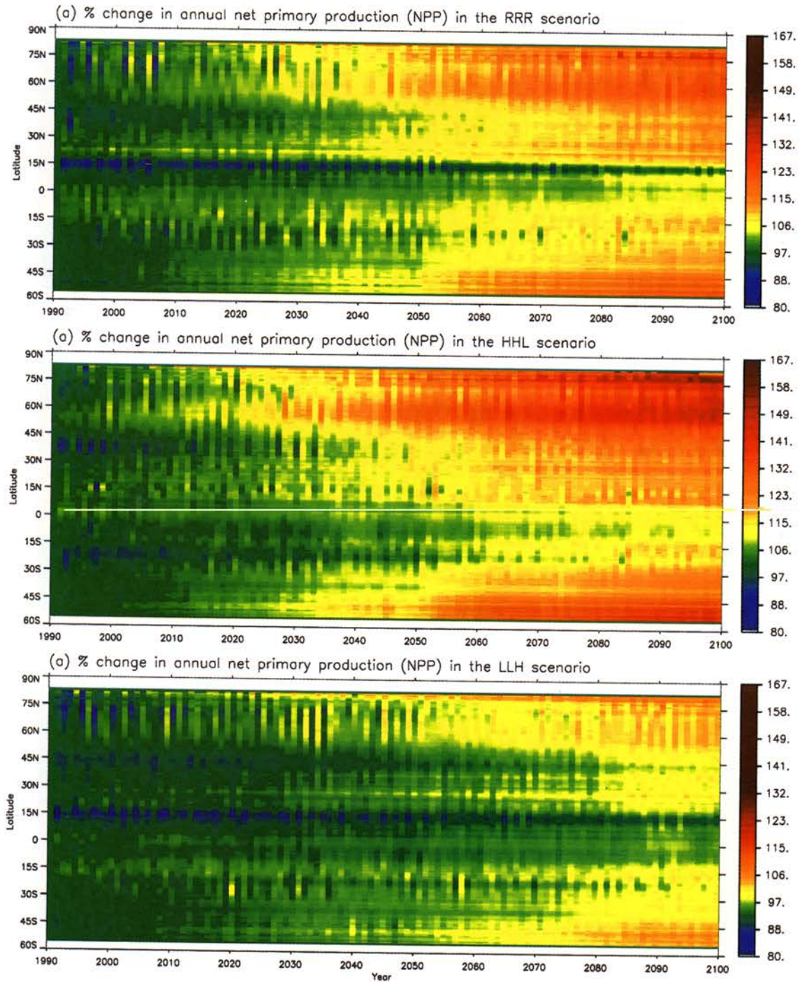
Plate 3. Percent changes of annual net primary production (NPP) along 0.5°-resolution latitudinal bands over the period of 1990-2100 in the RRR, HHL, and LLH transient climate change predictions. We used annual NPP in 1990 as the reference in calculating the percent change of annual NPP.
