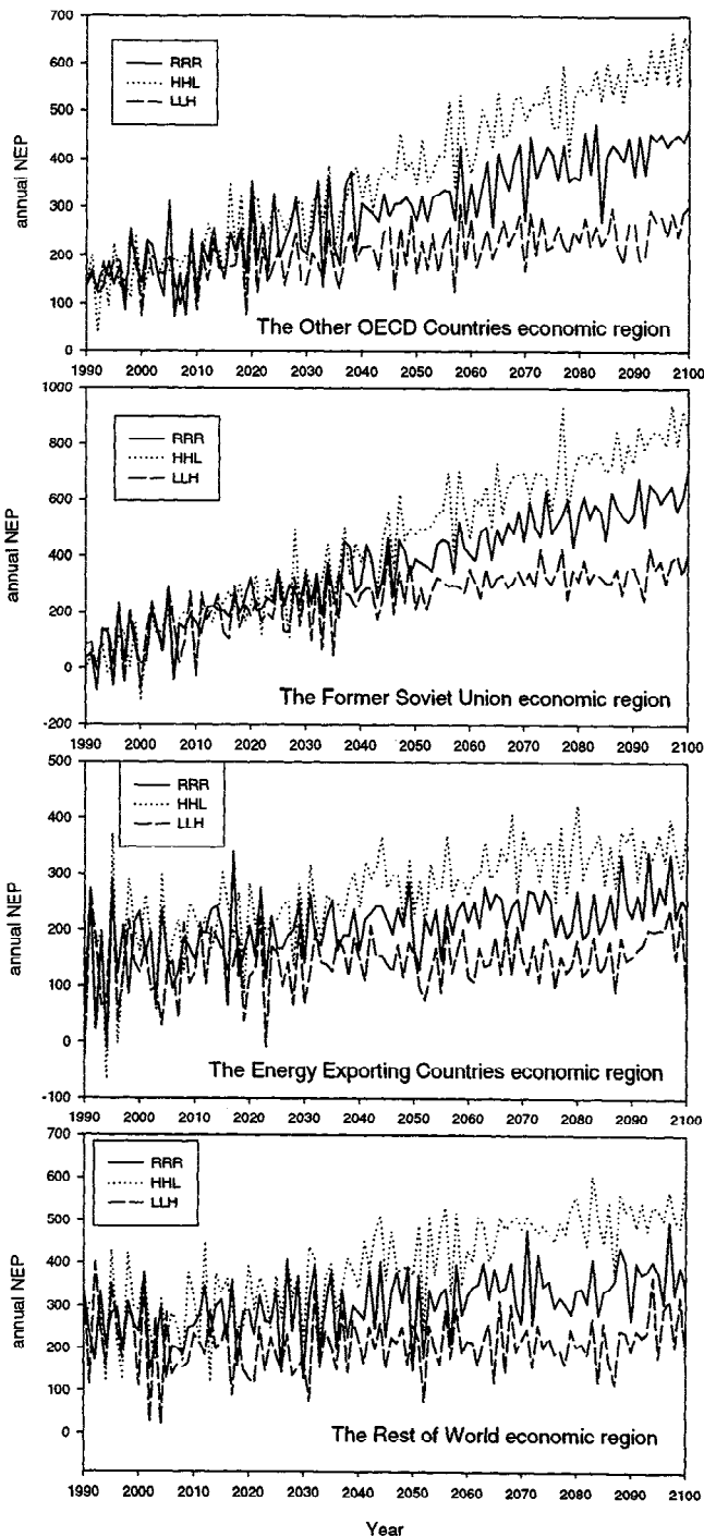
Figure 7. Temporal dynamics of annual net ecosystem production (NEP) ( 10^{12} \text{ g C yr}^{-1} ) among the four economic regions of the world over the period of 1990–2100 in the RRR, HHL, and LLH climate change predictions.
