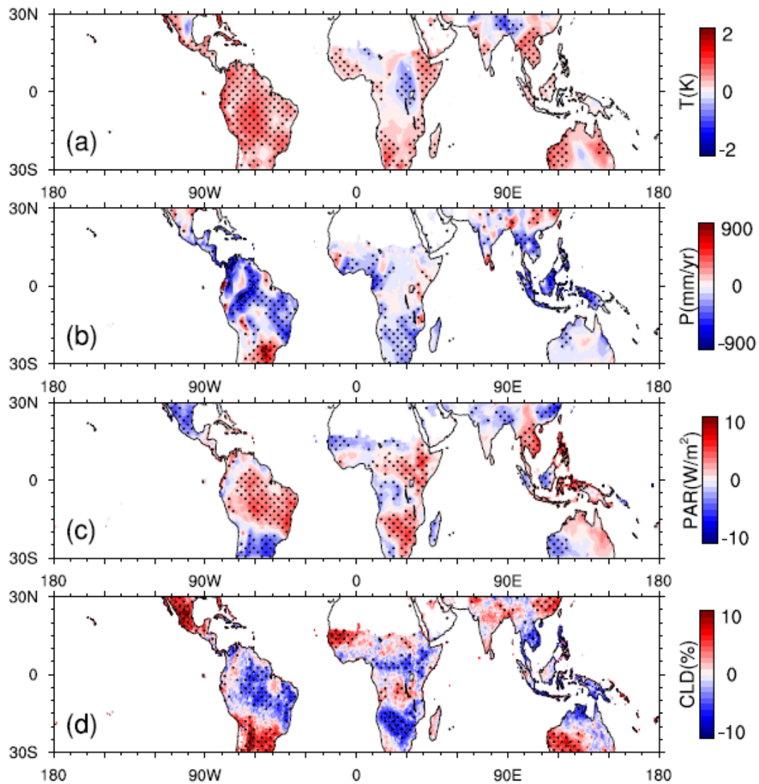
Figure 1. Spatial distributions of annual anomalies in (a) surface air temperature (K), (b) precipitation ( \text{mm year}^{-1} ), (c) photosynthesis active radiation ( \text{W m}^{-2} ) and (d) cloud fraction (%) of 2015 relative to the 15-year mean of 2001–2015. The stippled regions represent regions with anomalies larger than one interannual standard deviation.
