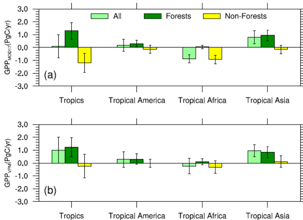
Figure 2. Total anomalies in (a) GPP MOD17 and (b) GPP VPM (PgC year -1 ) of 2015 relative to the 15-year mean of 2001–2015 for all grids (light green bars), forests-dominated (dark green bars) and non-forests-dominated (yellow bars) grids over the whole tropics, tropical America, Africa and Asia, respectively. The bars represent one standard deviation.
