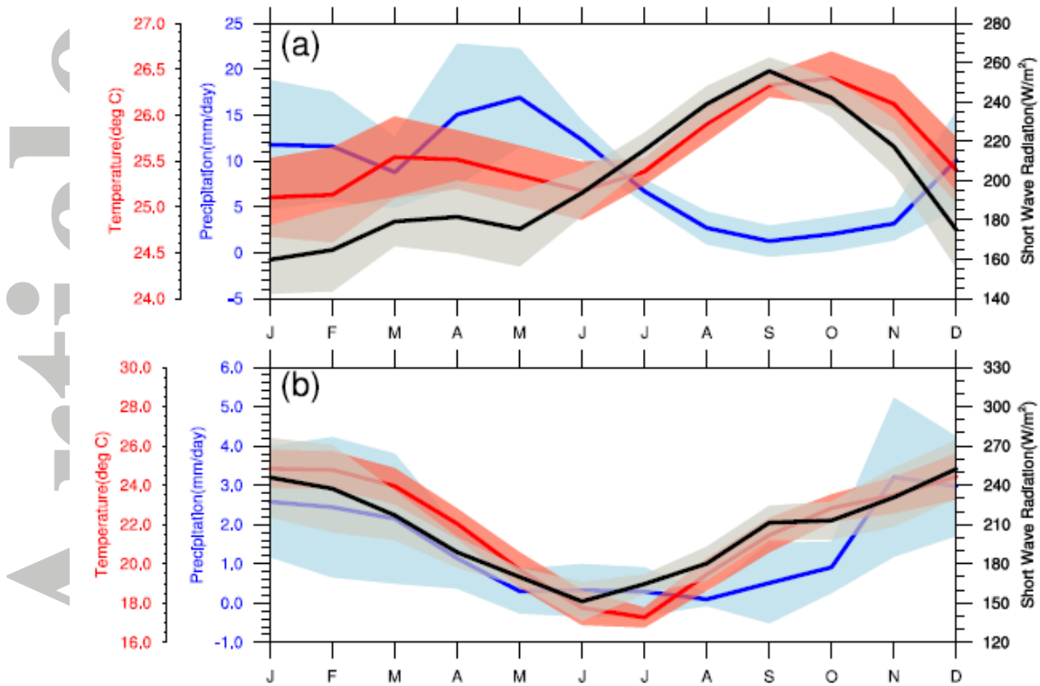
Figure 7. Seasonal variations of temperature (degree C, red lines), precipitation (mm, blue lines) and short wave radiation ( \text{W m}^{-2} , black lines) at sites (a) GF-Guy and (b) ZA-Kru. Lines represent the multi-year mean of 2004–2014 for (a) and 2000–2009 for (b), and the shaded areas represent one standard deviation.
