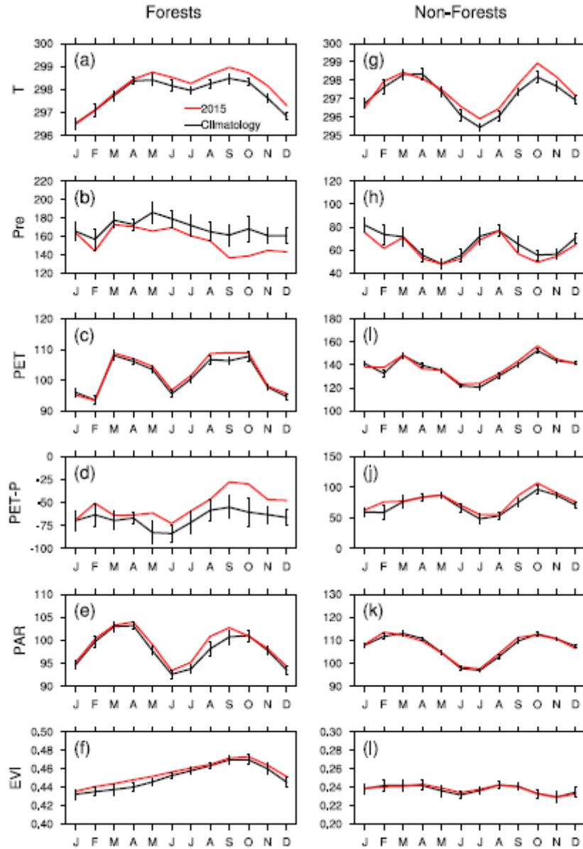
Figure 5. Seasonal variations in (a) surface temperature (K), (b) precipitation ( \text{mm month}^{-1} ), (c) potential evapotranspiration (PET; \text{mm month}^{-1} ), (d) water stress (PET-P; \text{mm month}^{-1} ), (e) photosynthesis active radiation (PAR; \text{W m}^{-2} ) and (f) EVI of 2015 (red lines) and the 15-year mean of 2001–2015 (black lines) in tropical forests-dominated regions. Patterns (g)–(l) are the same as (a)–(f), respectively, but in tropical non-forests-dominated regions. The bars represent one standard deviation.
