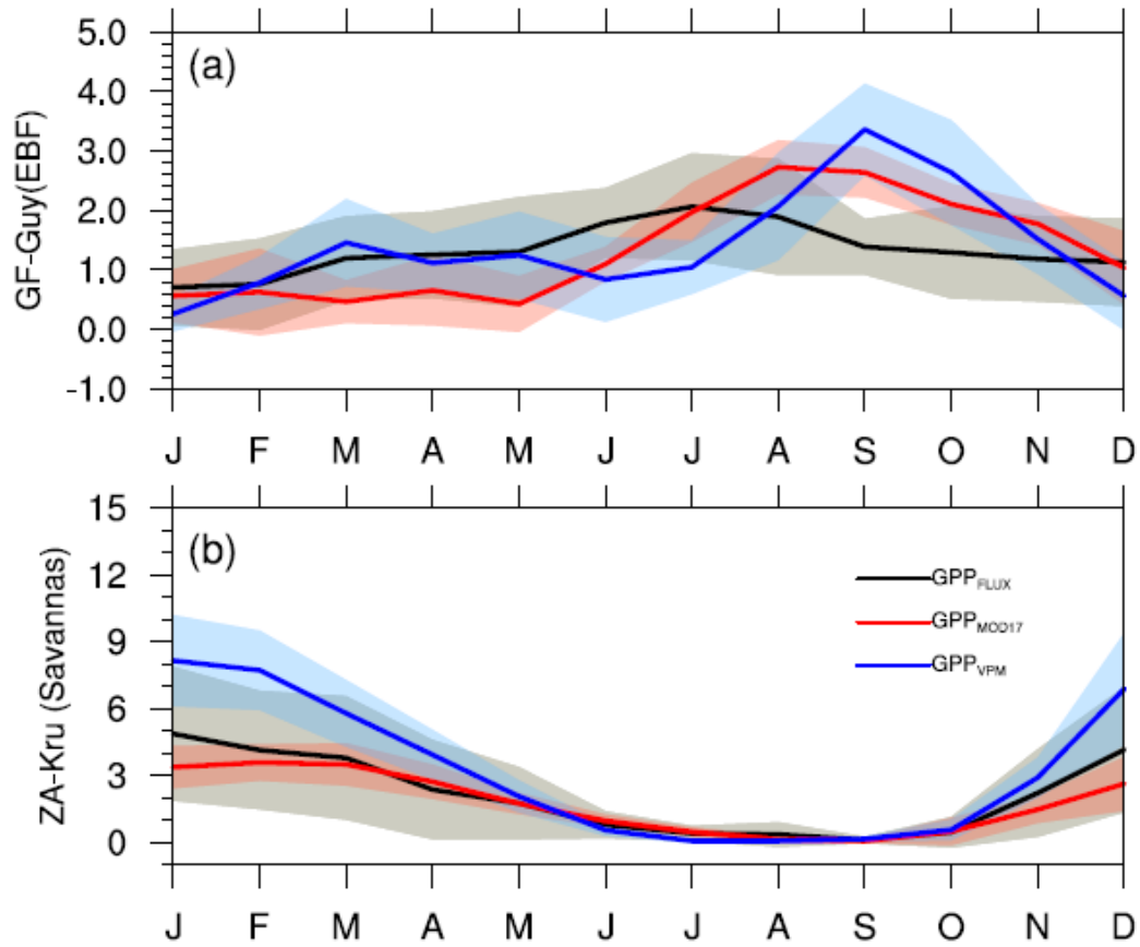
Figure 6. Seasonal variations of GPP FLUX (black lines), GPP MOD17 (red lines) and GPP VPM (blue lines) at sites (a) GF-Guy and (b) ZA-Kru. Values are derived by calculating differences between the GPP of each month and the minimum GPP of corresponding 12 months at each year. Lines represent the multi-year mean of 2004–2014 for (a) and 2000–2009 for (b), and the shaded areas represent one standard deviation. All units are gC m -2 day -1 .
