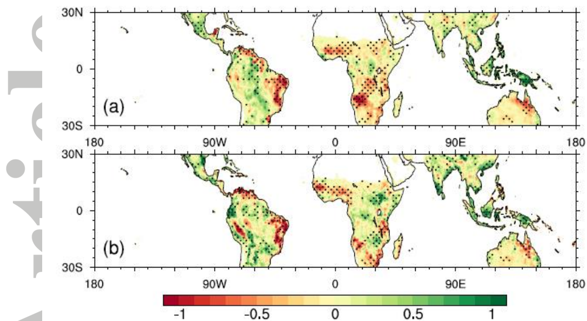
Figure 3. Spatial patterns of (a) GPP MOD17 and (b) GPP VPM anomalies ( \text{gC m}^{-2} \text{day}^{-1} ) in 2015 relative to the 15-year mean of 2001–2015. The stippled regions represent regions with anomalies larger than one interannual standard deviation.
