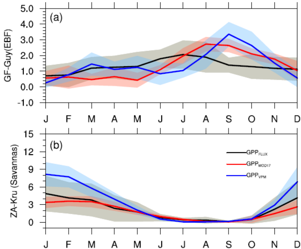
Figure 6. Seasonal variations of \text{GPP}_{\text{FLUX}} (black lines), \text{GPP}_{\text{MOD17}} (red lines) and \text{GPP}_{\text{VPM}} (blue lines) at sites (a) GF-Guy and (b) ZA-Kru. Values are derived by calculating differences between the GPP of each month and the minimum GPP of corresponding 12 months at each year. Lines represent the multi-year mean of 2004–2014 for (a) and 2000–2009 for (b), and the shaded areas represent one standard deviation. All units are \text{gC m}^{-2} \text{day}^{-1} .
