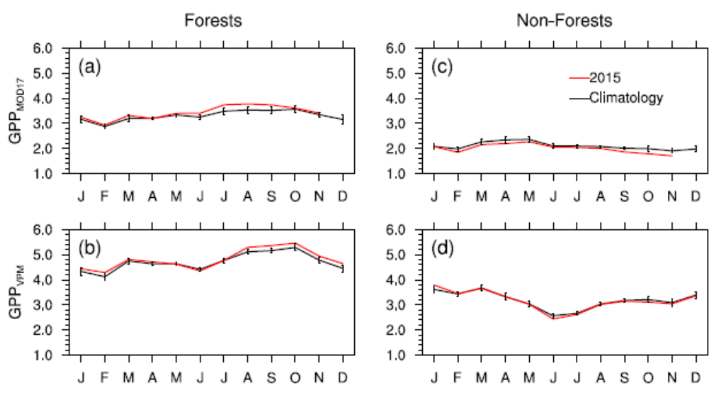
Figure 4. Seasonal variations in (a) GPP_{MOD17} ( PgC\ month^{-1} ) and (b) GPP_{VPM} ( PgC\ month^{-1} ) of 2015 (red lines) and the 15-year mean of 2001–2015 (black lines) in tropical forests-dominated regions. (c) and (d) are the same as (a) and (b), respectively, but in tropical non-forests-dominated regions. The bars represent one standard deviation.
