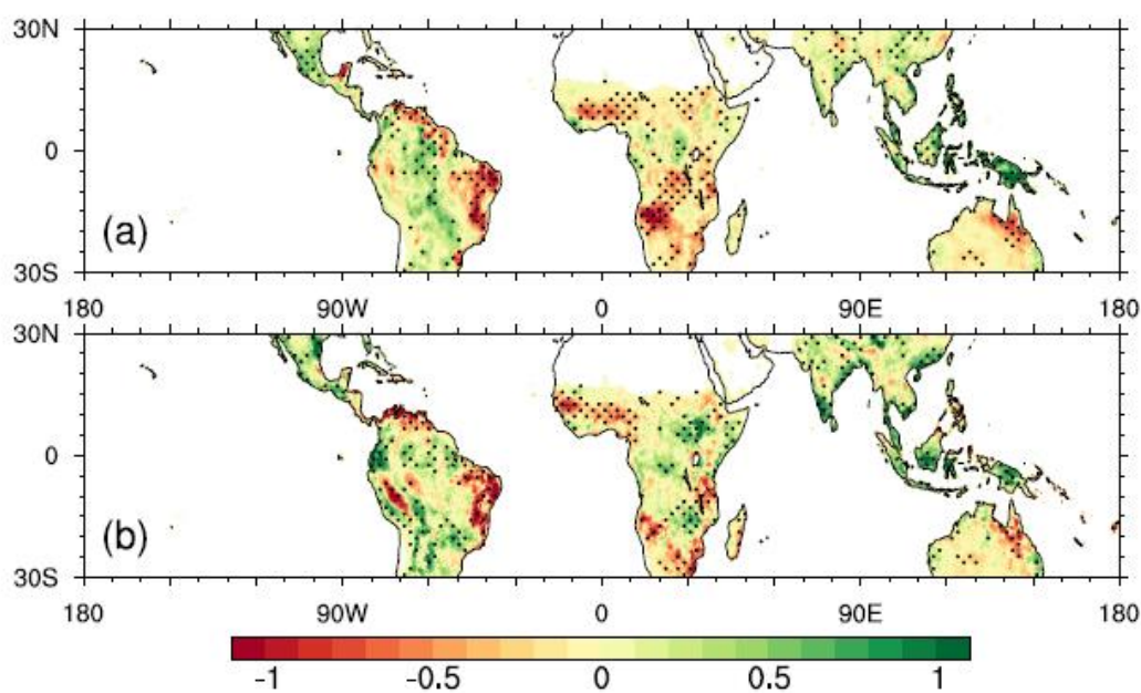
Figure 3. Spatial patterns of (a) \text{GPP}_{\text{MOD17}} and (b) \text{GPP}_{\text{VPM}} anomalies ( \text{gC m}^{-2} \text{ day}^{-1} ) in 2015 relative to the 15-year mean of 2001–2015. The stippled regions represent regions with anomalies larger than one interannual standard deviation.
