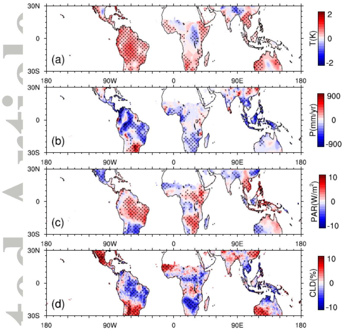
Figure 1. Spatial distributions of annual anomalies in (a) surface air temperature (K), (b) precipitation ( \text{mm year}^{-1} ), (c) photosynthesis active radiation ( \text{W m}^{-2} ) and (d) cloud fraction (%) of 2015 relative to the 15-year mean of 2001–2015. The stippled regions represent regions with anomalies larger than one interannual standard deviation.
