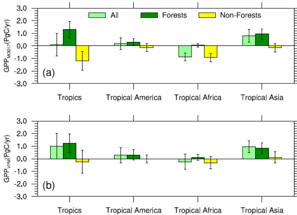
Figure 2. Total anomalies in (a) GPP_{MOD17} and (b) GPP_{VPM} ( PgC\ year^{-1} ) of 2015 relative to the 15-year mean of 2001–2015 for all grids (light green bars), forests-dominated (dark green bars) and non-forests-dominated (yellow bars) grids over the whole tropics, tropical America, Africa and Asia, respectively. The bars represent one standard deviation.
