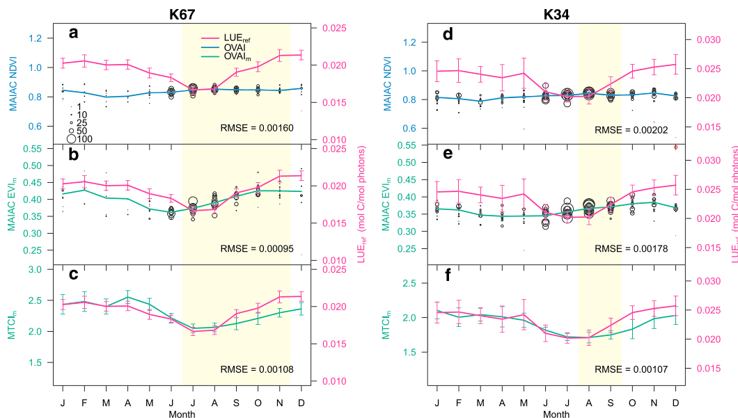
Figure 4. Comparing fPAR_{canopy} (NDVI) and approximation of fPAR_{chl} ( EVI_m , MTCI_m ) with LUE_{ref} at (a–c) K67 and (d–f) K34 sites in Amazon forest. EVI and NDVI data are calculated from MAIAC reflectance. Each circle in (a, b, d, and e) represents the average of all valid observations of vegetation indices for each year each month. The size of the circles represents the numbers of valid observations used. Some obvious outliers were colored in red and eliminated from further analysis. The blue and green lines in (a, b, d, and e) represent the observation numbers weighted averages of EVI or NDVI. The error bars for LUE_{ref} represent the standard error of mean. The error bars for MTCI_m in (c and f) represent the standard deviation for the period 2002 to 2012. The shades in light yellow represent dry season. Root-mean-square errors (RMSEs) are calculated based on regressions with zero intercept.
