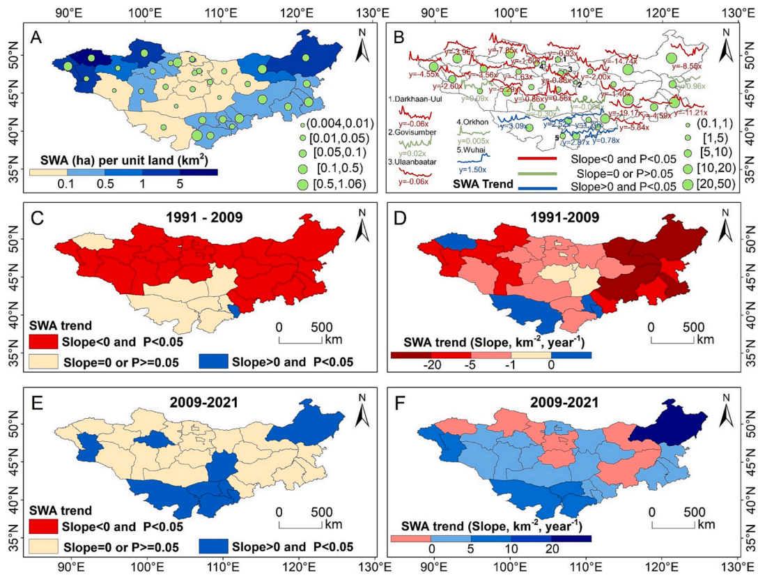
Fig. 8. Trends of SWA in the MP at the scale of the administrative region. (A) Annual mean SWA (ha) per unit land (km 2 ) and the standard deviation from 1991 to 2021; (B) Inter-annual variations and linear trends of SWA from 1991 to 2021; (C-D) Spatial patterns of linear trends of SWA from 1991 to 2009; (E-F) Spatial patterns of linear trends of SWA from 2009 to 2021.
