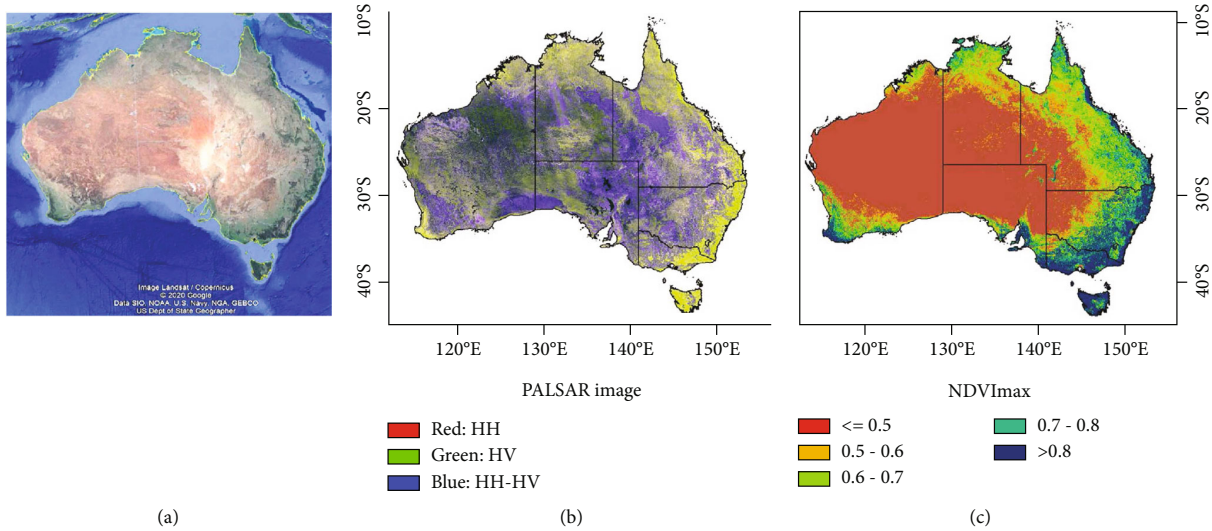
FIGURE 2: Spatial distribution of Google Earth image, PALSAR image, and the maximum Normalized Difference Vegetation Index (NDVImax) in Australia. (a) Google Earth image. (b) PALSAR false-color composite (red: HH, green: HV, and blue: HH-HV) in 2010. (c) The NDVImax image in 2010.
