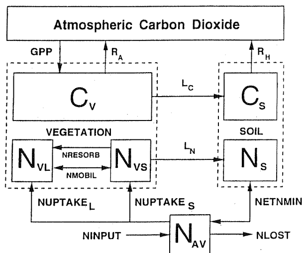
Figure 1. The Terrestrial Ecosystem Model (TEM). The state variables are carbon in the vegetation (C V ); structural nitrogen in the vegetation (N VS ); labile nitrogen in the vegetation (N VL ); organic carbon in soils and detritus (C S ); organic nitrogen in soils and detritus (N S ); and available soil inorganic nitrogen (N AV ). Arrows show carbon and nitrogen fluxes; GPP, gross primary production; R A , autotrophic respiration; R H , heterotrophic respiration; L C , litterfall carbon; L N , litterfall nitrogen; NUPTAKE S , nitrogen uptake into the structural nitrogen pool of the vegetation; NUPTAKE L , nitrogen uptake into the labile nitrogen pool of the vegetation; NRESORB, nitrogen resorption from dying tissue into the labile nitrogen pool of the vegetation; NMOBIL, nitrogen mobilized between the structural and labile nitrogen pools of the vegetation; NETNMIN, net nitrogen mineralization of soil organic nitrogen; NINPUT, nitrogen inputs from outside the ecosystem; and NLOST, nitrogen losses from the ecosystem.
