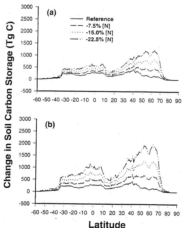
Figure 7. Sensitivity to 7.5, 15.0, and 22.5% decreases in vegetation nitrogen concentration for the latitudinal distributions of soil carbon responses to doubled CO 2 as estimated by the Terrestrial Ecosystem Model for simulations in which changes in vegetation nitrogen concentration are (a) uncoupled from decomposition dynamics and (b) coupled to decomposition dynamics. The doubled CO 2 responses are for a change in atmospheric CO 2 from 340 to 680 ppmv with no change in climate from contemporary. The latitudinal distribution of the reference response of soil for no change in vegetation nitrogen concentration is shown for comparison. The resolution of carbon storage responses is 0.5° latitude.
