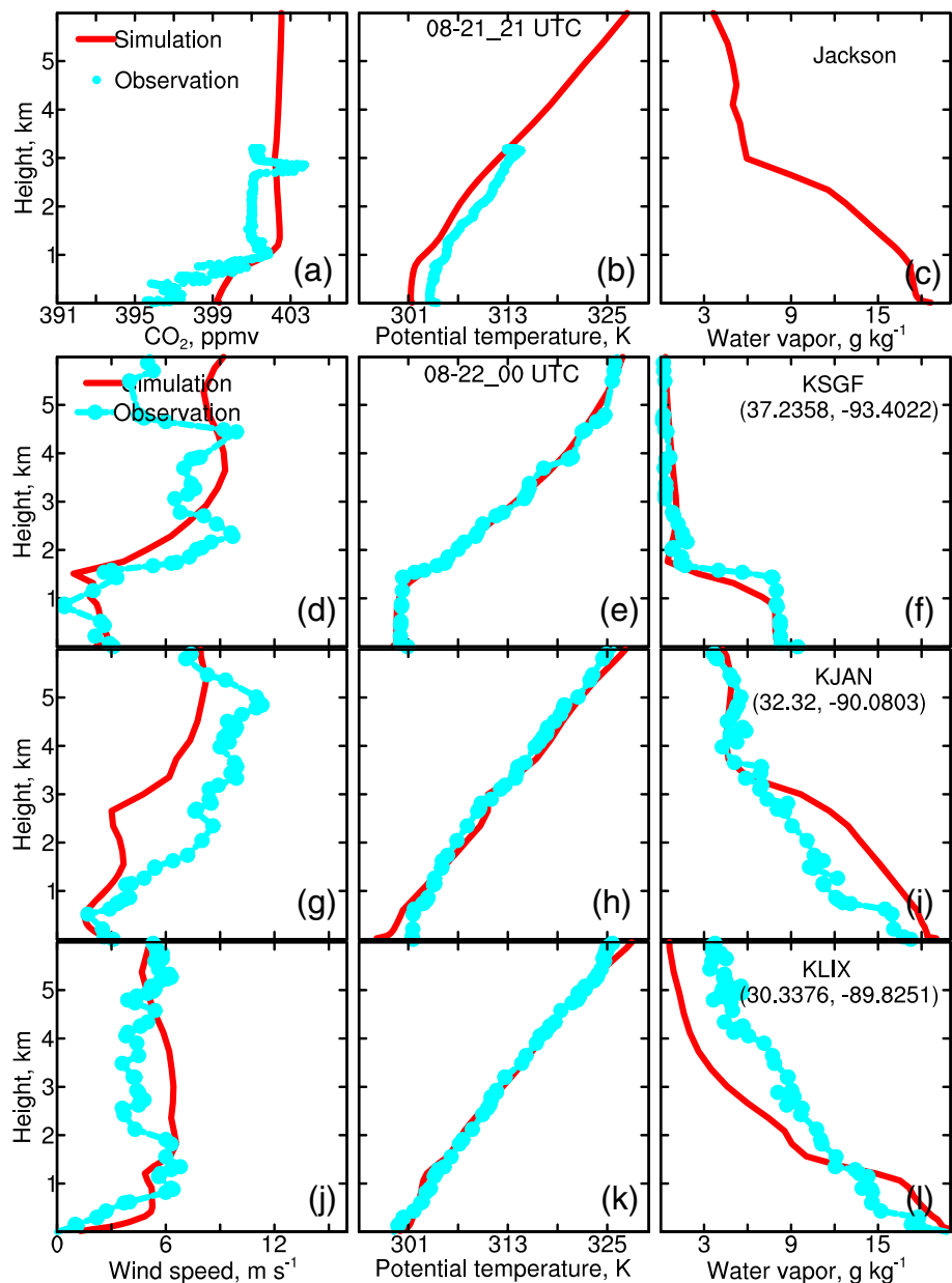
Figure 27. (a–c) Profiles of \text{CO}_2 , potential temperature ( \theta ), and water vapor mixing ratio simulated at 2100 UTC and observed during B200 taking off at \sim 2030 UTC on 21 August over the Jackson Airport ( 32.3163^\circ\text{N} , 90.072^\circ\text{W} ), and profiles of (left to right) wind speed, \theta , and water vapor mixing ratio at 0000 UTC on 22 August simulated and observed at sounding sites: (d–f) KSGF, (g–i) KJAN, and (j–l) KLIX, which are marked on Figure 26a. Note that water vapor is not available from B200 during this flight.
