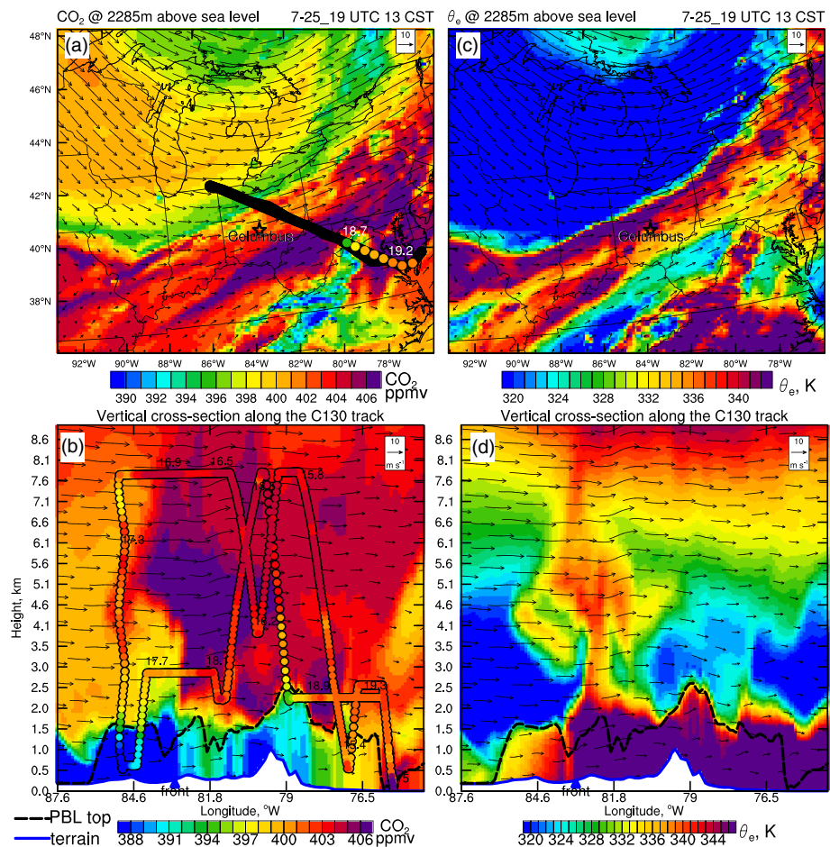
Figure 19. (a, c) Horizontal (at 2,285 m above sea level) and (b, d) vertical cross sections of CO 2 and equivalent potential temperature ( \theta_e ) at 1900 UTC on 25 July simulated by WRF-VPRM, overlaid with C130 aircraft CO 2 data. Note that the flight path and CO 2 data at 2,285 m above sea level is marked in panel a. The black segment of the flight path means the path is not at 2,285 m. Each flight took a few hours, the UTC time is marked along the flight path, while the cross section of simulated CO 2 is an instantaneous snapshot. C130 flew over the Appalachian Mountains at ~1900 UTC. The simulated front location is marked with a blue triangle in panels (b) and (d).
