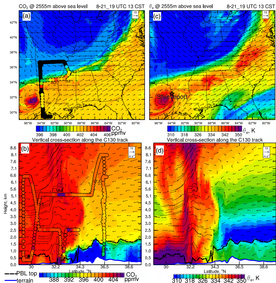
Figure 25. (a, c) Horizontal (at ~2,555 m above sea level) and (b, d) vertical cross sections of CO 2 and equivalent potential temperature ( \theta_e ) through the straight south-north oriented flight path at 1900 UTC on 21 August simulated by WRF-VPRM, overlaid with C130 aircraft CO 2 data. Note that the flight path and CO 2 data at ~2,555 m above sea level is marked in panel (a). The UTC time is marked along the flight path. In panel (b), the data not on the straight south-north oriented flight path are not shown.
