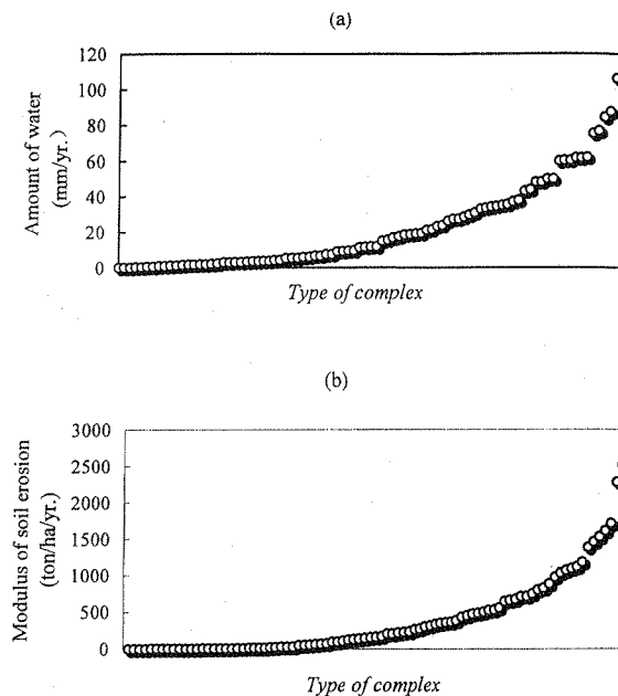
Fig. 2. (a) The capacities of water conservation of the complexes. Here, minimum is the complex of CRP–RCS–SA > 25°; maximum is the complex of MIX–YBS–SA < 15°. (b) The moduli of soil erosion of the complexes. Here, minimum is the complex of MIX–YBS–SA < 15°; maximum is the complex of CRP–RCS–SA > 25°.
