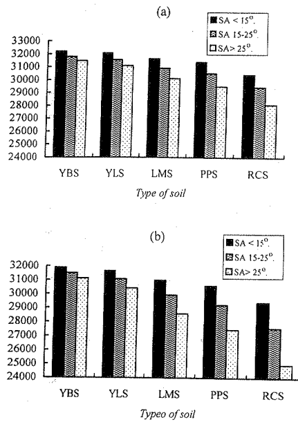
Fig. 3. The economic values of every complex with (a) MIX and (b) CON.
