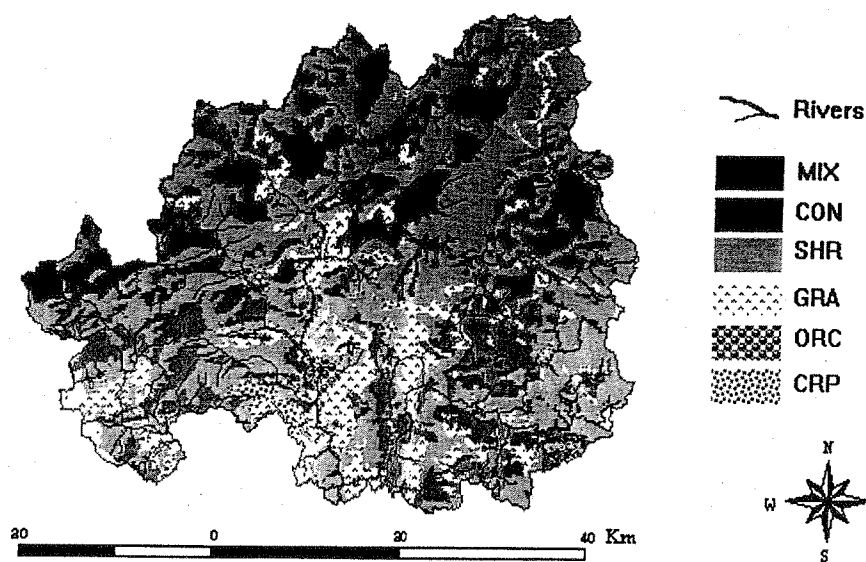
Fig. 1. Vegetation in Xingshan County.
