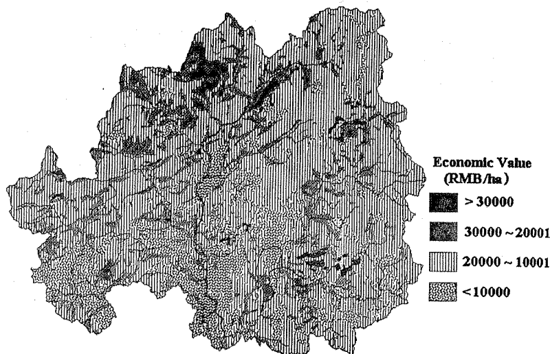
Fig. 4. The spatial distribution of economic values of forest ecosystem services in Xingshan County.
