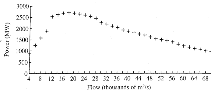
FIG. 4. The relationship between water flow in the Yangtze River and power generation at the Gezhouba Hydroelectric Power Plant.
