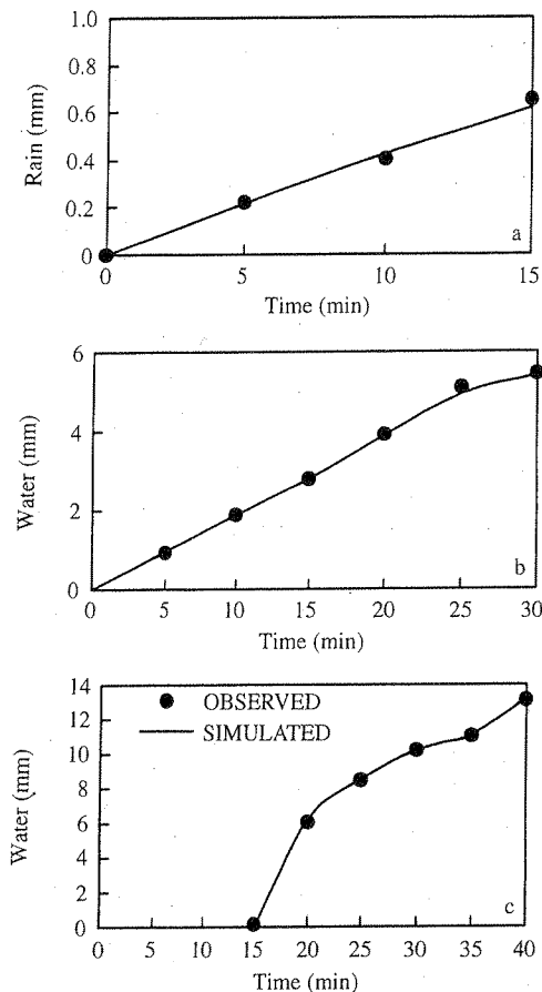
FIG. 5. The comparison between the observed and simulated capacity of water flow regulation during a rainfall event by the MIX + YBS + slope angle < 15^\circ complex in Xingshan County (see Table 2 for reference): (a) rain interception by forest canopy, (b) water absorption by litter, and (c) underground water storage.
