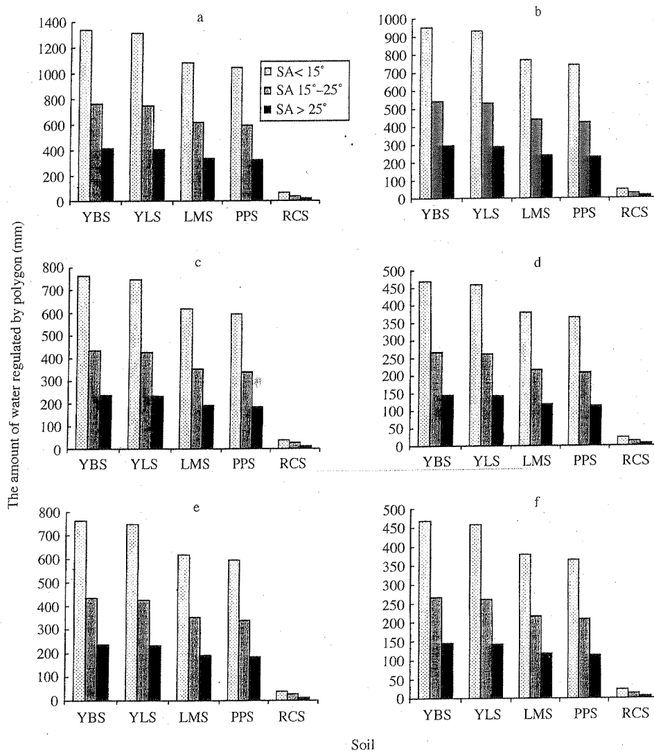
FIG. 7. The comparison among the simulated capacities of water flow regulation by all 90 types of vegetation–soil–slope complexes in Xingshan County (see Table 1 and 2 for reference), as grouped by vegetation types: (a) MIX, (b) CON, (c) SHR, (d) GRA, (e) ORC, and (f) CRP. SA = slope angle.
