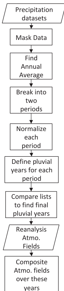
FIG. 3. Description of the workflow used to create each composite type. EGHa stands for EGH anomalies and “Atmo.” is used in place of “atmospheric.”
