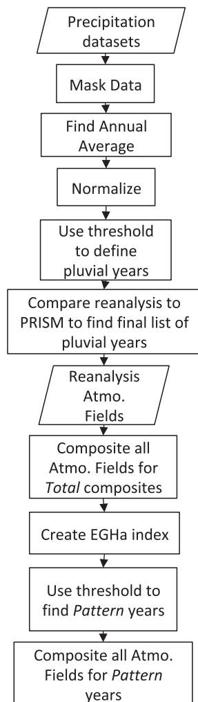
FIG. 3. Description of the workflow used to create each composite type. EGHa stands for EGH anomalies and “Atmo.” is used in place of “atmospheric.”
