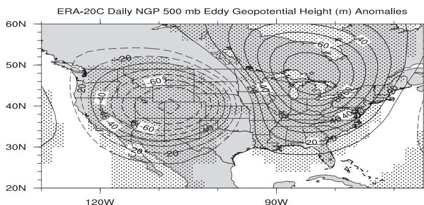
FIG. 8. Composite 500-mb EGH anomalies (m) for daily heavy rain events for the (a) SGP and (b) NGP. Contours are from -80 to 80 m with intervals of 10 m, and values that are statistically significant at the 90\% level are stippled. Negative contours are dashed, and solid contours represent positive values.
