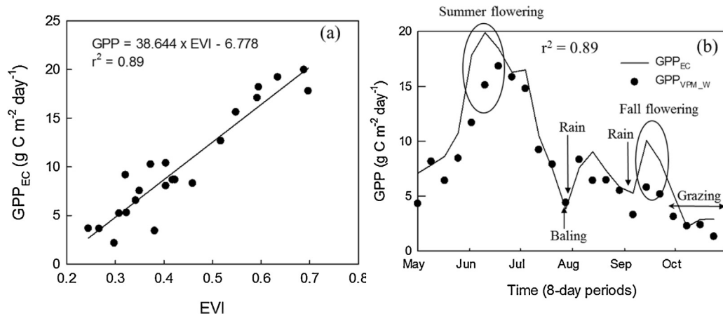
Fig. 11. (a) Relationship between enhanced vegetation index (EVI) and gross primary production ( GPP_{EC} ). (b) Comparison between gross primary production (GPP) from VPM simulation and EC measurement ( GPP_{VPM,W} and GPP_{EC} ).
